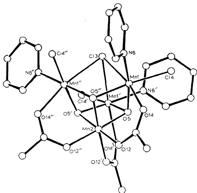
Figure 4. The structure of complex 5 ( R = \text{Me} ): \text{Mn}(1)\cdots\text{Mn}(2) , 2.815 (2) Å; \text{Mn}(1)\cdots\text{Mn}(1') , 3.272 (2) Å. (Reprinted with permission from ref 19. Copyright 1988 VCH (Weinheim).)
