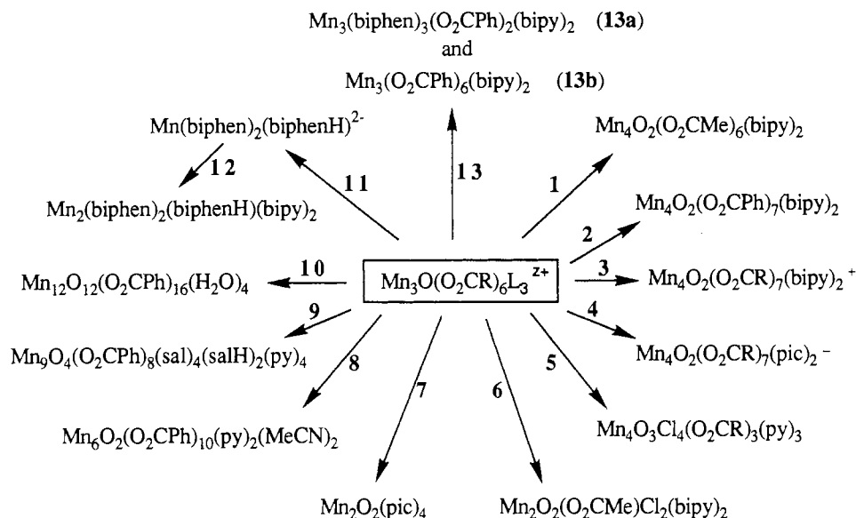
Figure 2. The established transformations of [\text{Mn}_3\text{O}] starting materials. Conditions: 1, z = 0 , bipy; 2, z = 0 , bipy; 3, R = Me, Et, or Ph, z = 1 , bipy; 4, R = Me or Ph, z = 1 , Na(pic); 5, R = Me or Et, z = 1 , \text{Me}_3\text{SiCl} ; 6, z = 1 , \text{Me}_3\text{SiCl} , bipy; 7, R = Me, z = 1 , \text{Me}_3\text{SiCl} , Na(pic); 8, z = 0 , phenol or NaACN; 9, z = 0 , salH 2 ; 10, z = 1 , N - n - \text{Bu}_4\text{MnO}_4 , py, \text{PhCO}_2\text{H} ; 11, R = Ph, z = 1 , biphenH 2 , NEt 3 ; 12, bipy; 13, z = 0 , biphenH 2 , NEt 3 , bipy. For reactions 1, 3–7, 10, and 11, L_3 = (\text{py})_3 ; for reactions 2, 8, 9, and 13, L_3 = (\text{py})_2(\text{H}_2\text{O}) . The identity of R is not specified when obvious from the product. The reaction solvent is MeCN unless otherwise stated.
