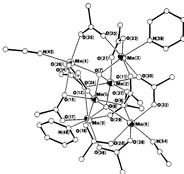
Figure 6. The structure of complex 8. \text{Mn}(1)\cdots\text{Mn}(2) , 2.820 (3) Å; \text{Mn}(1)\cdots\text{Mn}(3,4,5,6) , 3.139–3.543 Å; \text{Mn}(2)\cdots\text{Mn}(3,4,5,6) , 3.159–3.507 Å; \text{Mn}(3)\cdots\text{Mn}(4) , 3.732 (3) Å; \text{Mn}(5)\cdots\text{Mn}(6) , 3.824 (3) Å.
