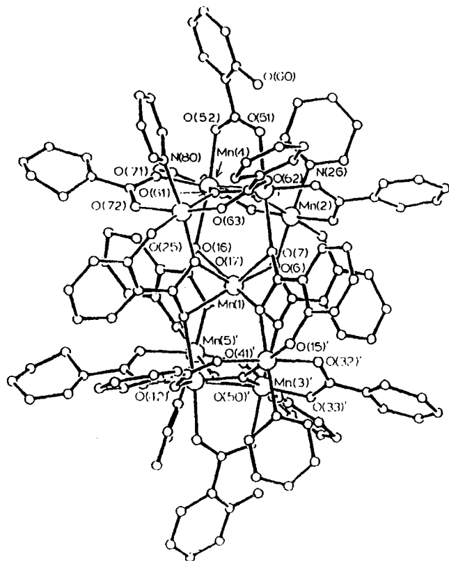
Figure 8. The structure of complex 12: Mn(1)···Mn(2), 3.182 (6) Å. (Reprinted with permission from ref 20a. Copyright 1988 Royal Society of Chemistry.)
