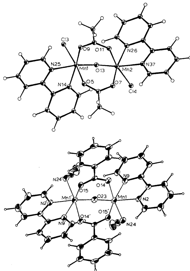
Figure 10. The structures of complex 14 (top) and complex 15 (bottom). For 14 : Mn(1)···Mn(2), 3.153 (3) Å. For 15 : Mn(1)···Mn(1'), 3.153 (4) Å.
