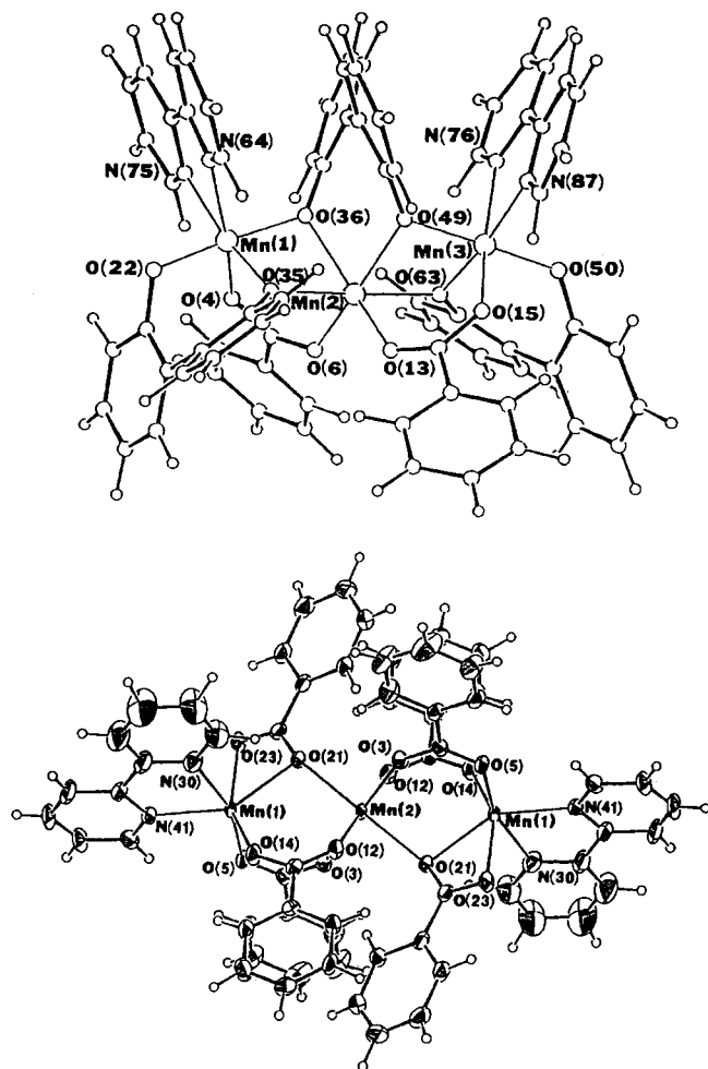
Figure 9. The structures of complex 13a (top) and complex 13b (bottom). For 13a : Mn(1)···Mn(2), 3.143 (3) Å; Mn(2)···Mn(3), 3.139 (3) Å. For 13b : Mn(1)···Mn(2), 3.588 (2) Å.
