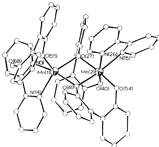
Figure 8. The structure of complex 12: Mn(1)···Mn(2), 3.182 (6) Å. (Reprinted with permission from ref 20a. Copyright 1988 Royal Society of Chemistry.)
