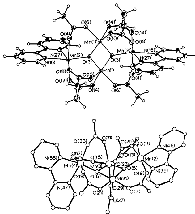
Figure 3. The structures of complexes 1 (top) and 3 (bottom). For 1: Mn(1)···Mn(1'), 2.779 (1) Å; Mn(1)···Mn(2), 3.288 (1) Å; Mn(1)···Mn(2'), 3.481 (1) Å. For 3: Mn(1)···Mn(3), 2.848 (5) Å; Mn(1)···Mn(2), 3.312 (5) Å; Mn(2)···Mn(3), 3.371 (5) Å; Mn(3)···Mn(4), 3.299 (5) Å; Mn(1)···Mn(4), 3.385 (5) Å.
