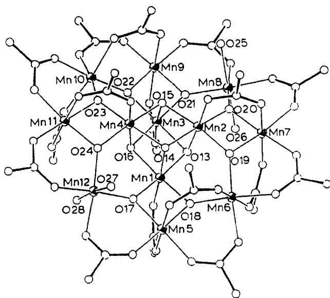
Figure 7. The structures of complex 9 (top) and 10 (bottom). For 9: Mn(1)···Mn(2,3,4,5), 3.814–3.983 Å; Mn(2)···Mn(3), 3.406 (6) Å; Mn(2)···Mn(4), 3.443 (6) Å; Mn(3)···Mn(5), 3.408 (6) Å; Mn(4)···Mn(5), 3.425 (6) Å; Mn(3)···Mn(4), 2.817 (6) Å. For 10: Mn···Mn distances in the central cube, 2.817–2.981 Å; Mn(1)···Mn(5), 2.809 (7) Å; Mn(2)···Mn(7), 2.775 (7) Å; Mn(3)···Mn(9), 2.803 (7) Å; Mn(4)···Mn(11), 2.813 (7) Å.
