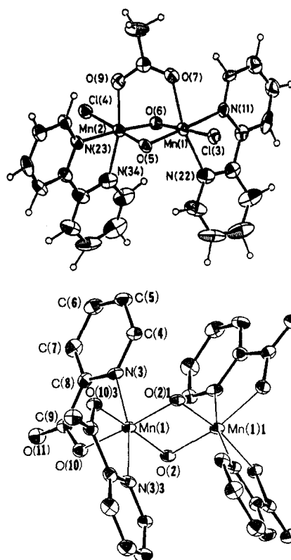
Figure 5. The structures of complex 6 (top) and complex 7 (bottom). For 6: \text{Mn}(1)\cdots\text{Mn}(2) , 2.667 (2) Å. For 7: \text{Mn}(1)\cdots\text{Mn}(11) , 2.747 (2) Å. (Reprinted with permission from ref 20a. Copyright 1988 Royal Society of Chemistry.)
